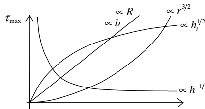
Fig. 6. Influence of geometry on maximum shearing stress.
