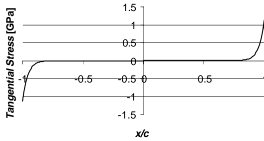
Fig. 3. Tangential stress.
