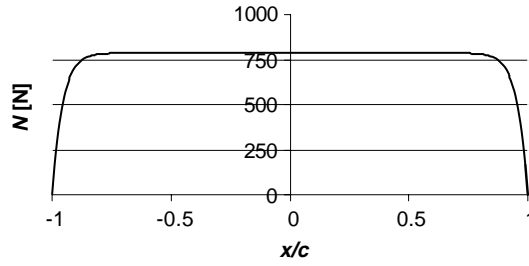
Fig. 2. Axial load.
