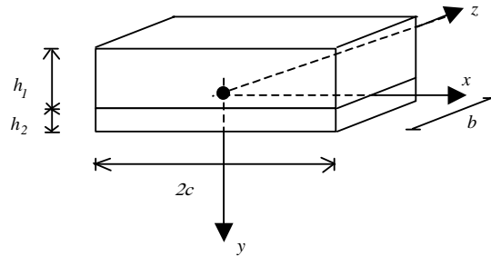
Fig. 1. Composite structure.
